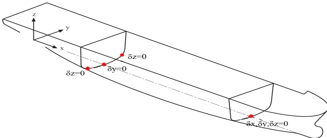
Figure 2.2.3: Boundary conditions
