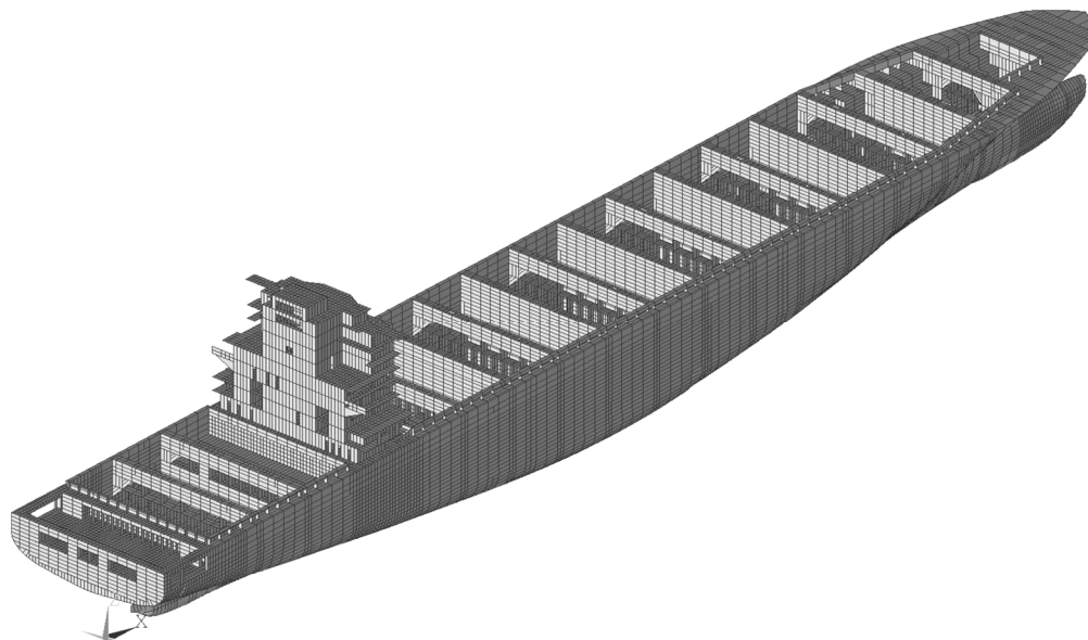
Figure 2.2.1 (b): Full ship model of a Container ship
