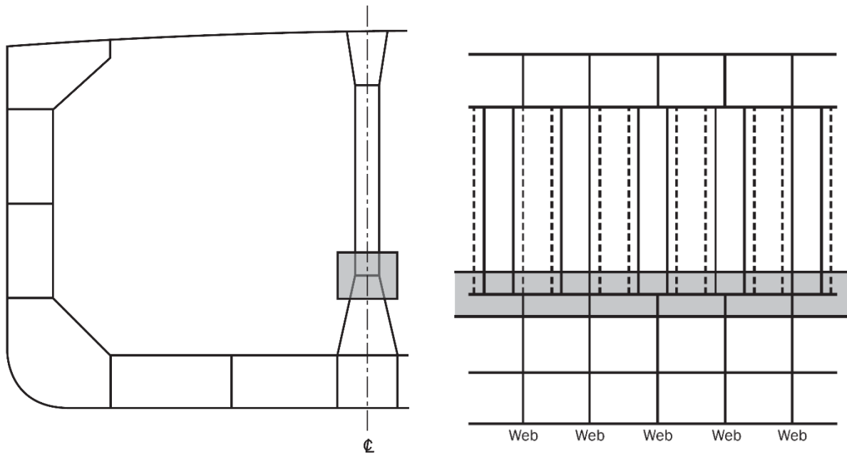
Figure 4.2.6: Mandatory area connection between corrugation and adjoining stool
