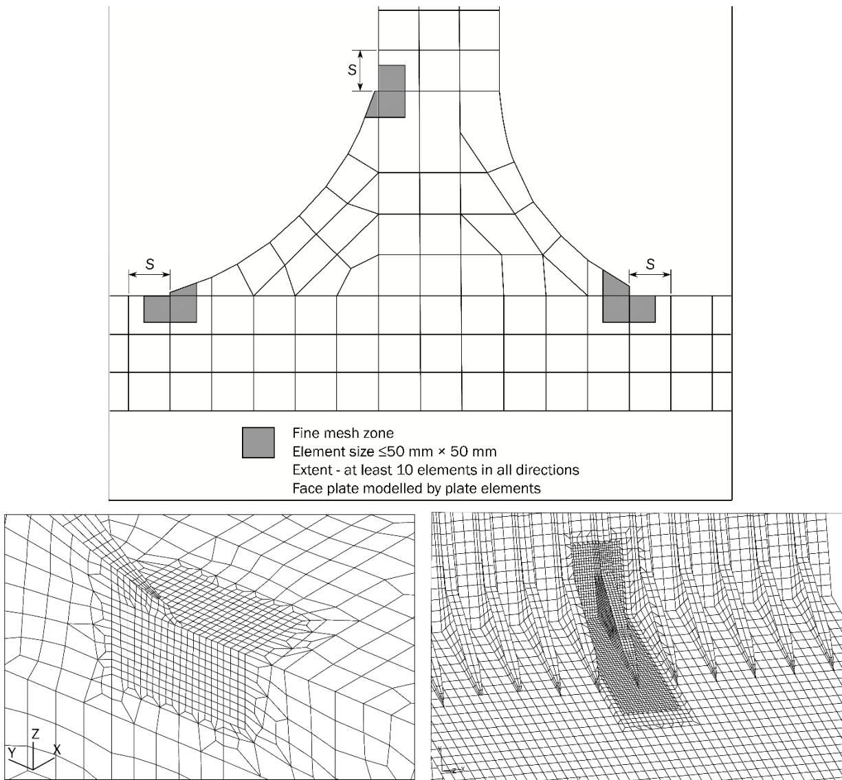
Figure 4.3.4 (b): Fine mesh zone around bracket toe
