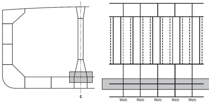
Figure A.1.1 (a): Screening areas at connections of lower stool to inner bottom and hopper tank
