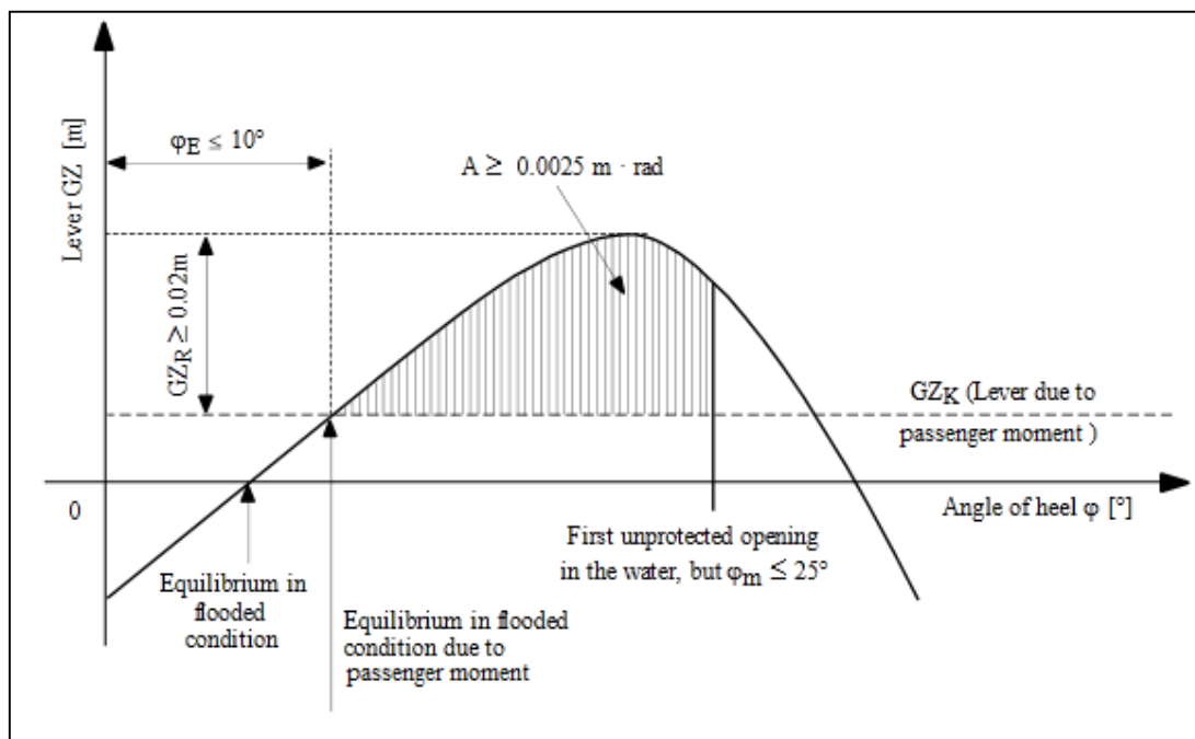
Figure 4.5: Damage Stability
