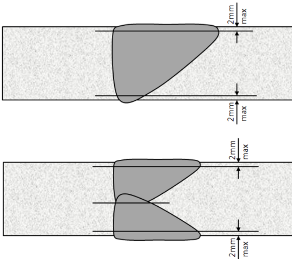
Fig. A 1 Examples of hardness test with rows of indentations in butt welds
