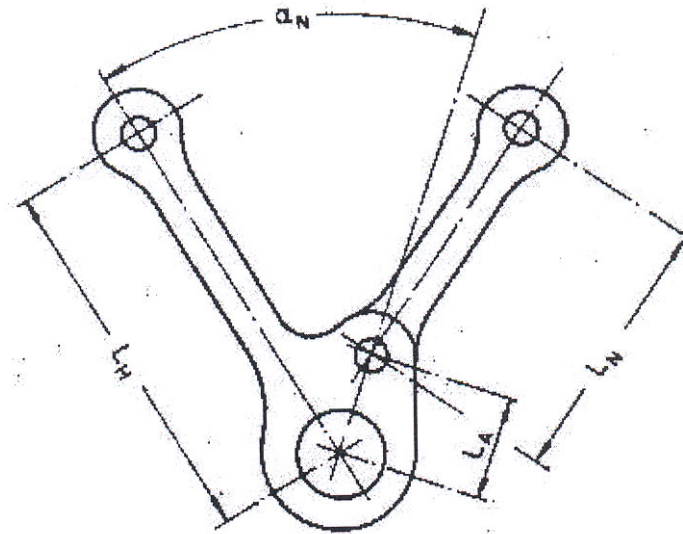
Fig. 2 : Articulated-type connecting-rod
