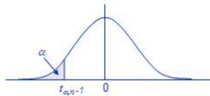
Figure 2.1. Student's t -distribution
