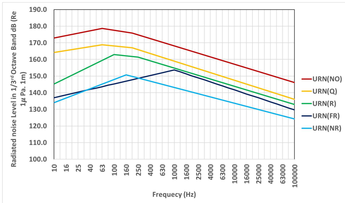
Fig. 3.2.2: URN Notations
